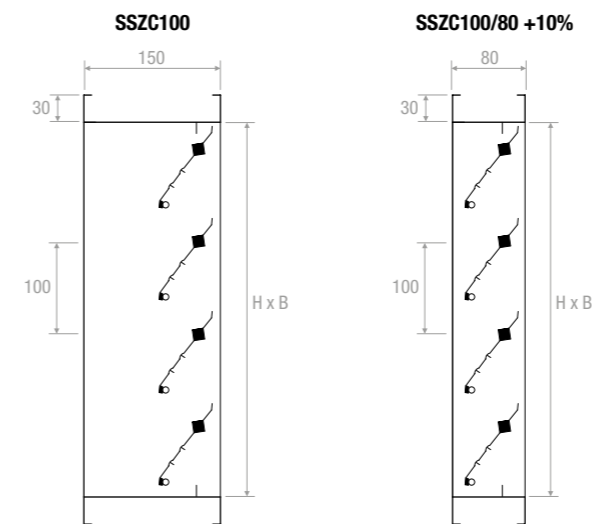
Alette coniugate +30% Blade with conjugate operation +30%
